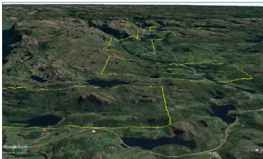
Figure 4-3 Oblique 3D view from Google Earth over the Bjerkreim licence areas, looking east
