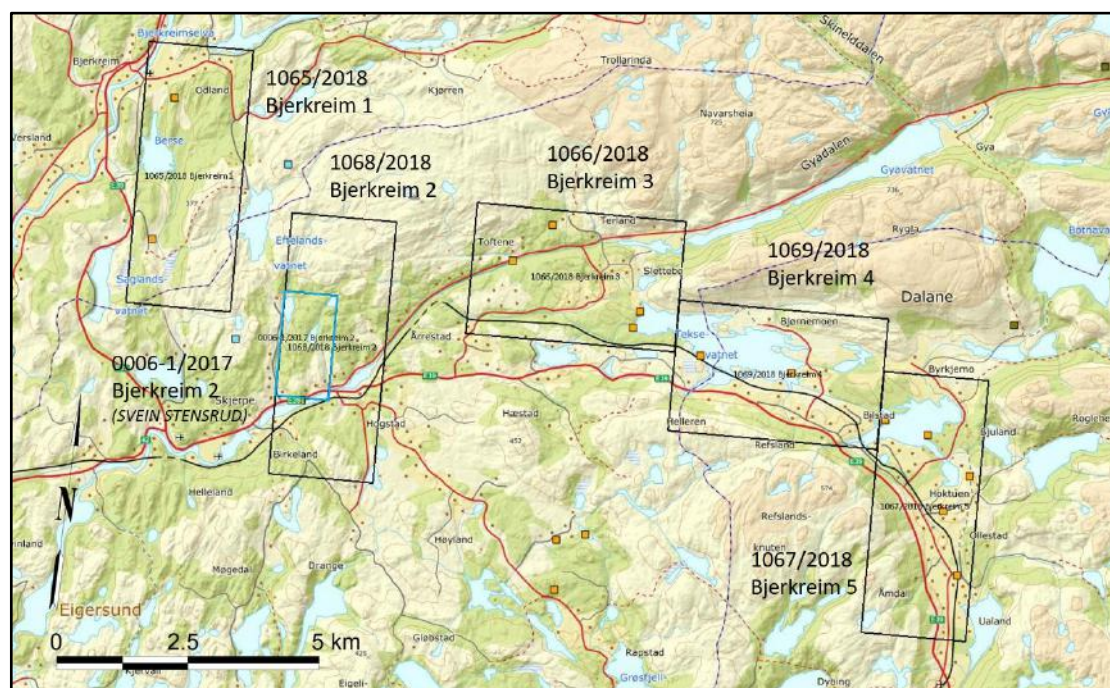
Figure 4-1 Location of the five NMP licences in the Bjerkreim area
