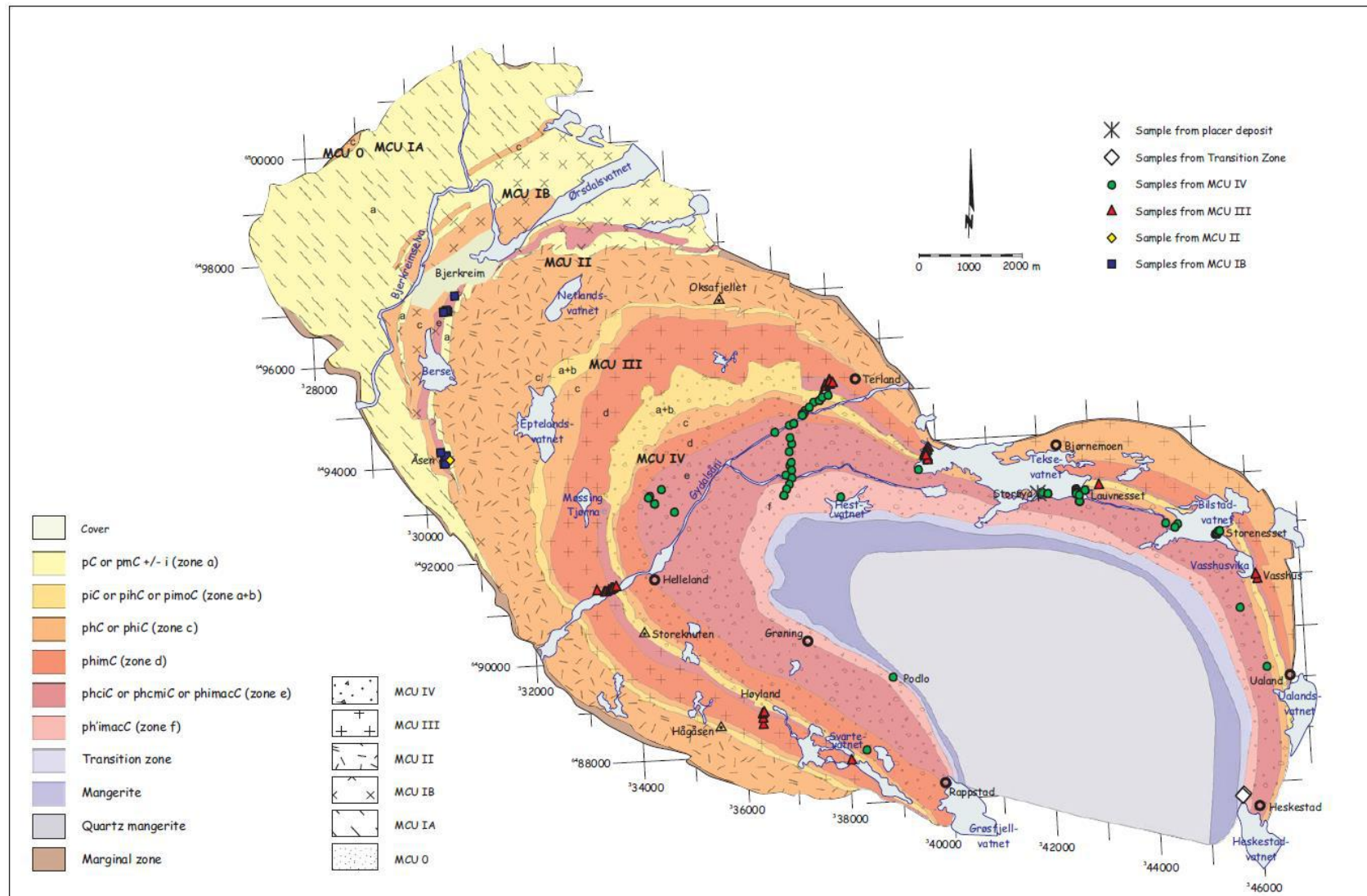
Figure 4-9 Geological map of the Bjerkreim lobe highlighting the megacyclic units and their constituent zones
